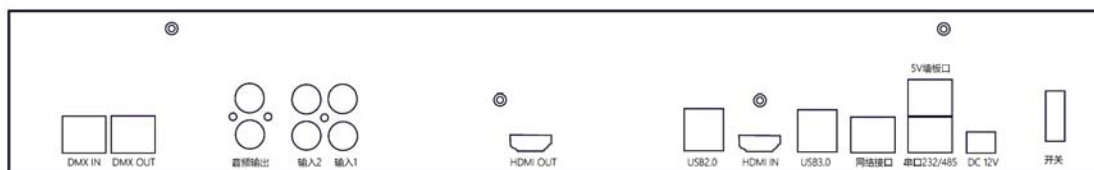
K-Shock T4 Backplane Interface Diagram
